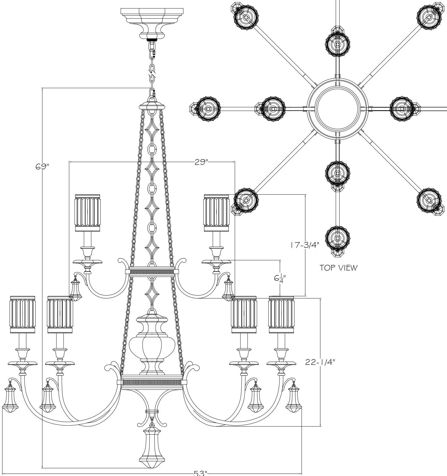
FRONT VIEW
